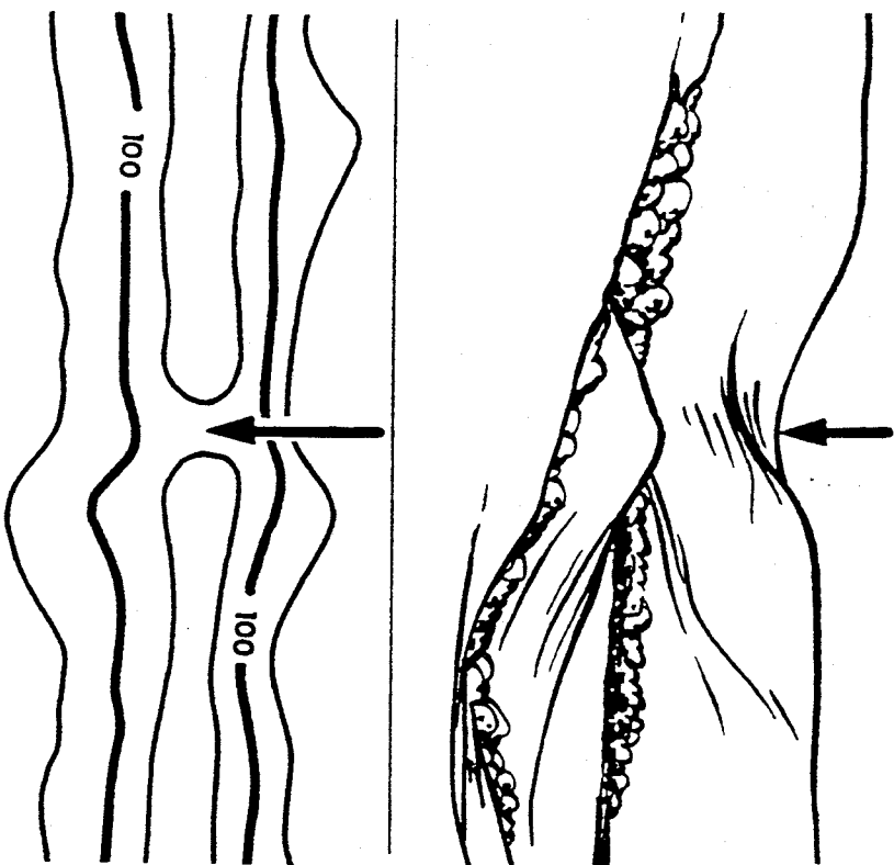
A saddle is a lower elevation between two knolls or ridges.
